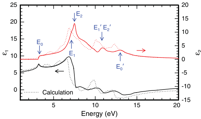
FIG. 6. (Color online) Real ( \epsilon_1 ) and imaginary ( \epsilon_2 ) parts of the dielectric function of c-GaN from 1 to 20 eV. Experimental data recorded at 295 K (continuous curves) are compared to theoretical calculations (dotted traces) reported in Ref. 43.
